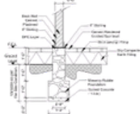
FOOTING F2 SCALE: 1/2"=1'-0" (AS SHOWN)
