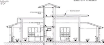
SECTION F-F scale 1/8"=1'-0"
