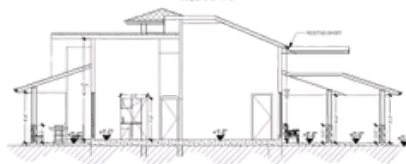
SECTION E-E scale 1/8"=1'-0"
