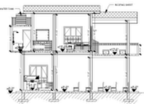
SECTION A-A scale 1/8"=1'-0"
