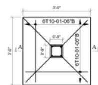
COLUMN FOOTING SCALE - 2 FT. TO AN IN.
