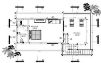
FIRST FLOOR PLAN scale 1/8"=1'-0"
