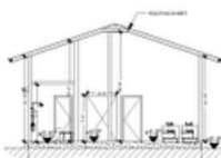
SECTION B-B scale 1/8"=1'-0"
