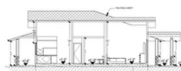
SECTION D-D scale 1/8"=1'-0"
