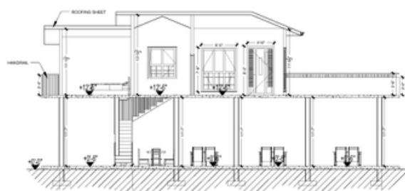
SECTION F-F scale 1/8"=1'0"
