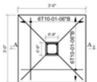
COLUMN FOOTING C1 SCALE - 1/8"=1'0"
