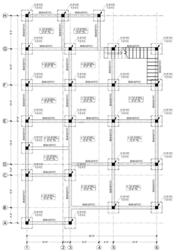
BEAM & COLUMN LAYOUT GROUND FLOOR scale 3/16"=1'0"
