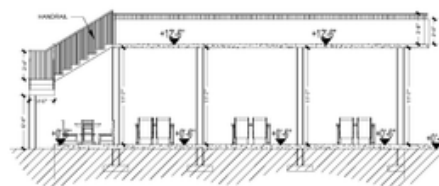
SECTION G-G scale 1/8"=1'0"
