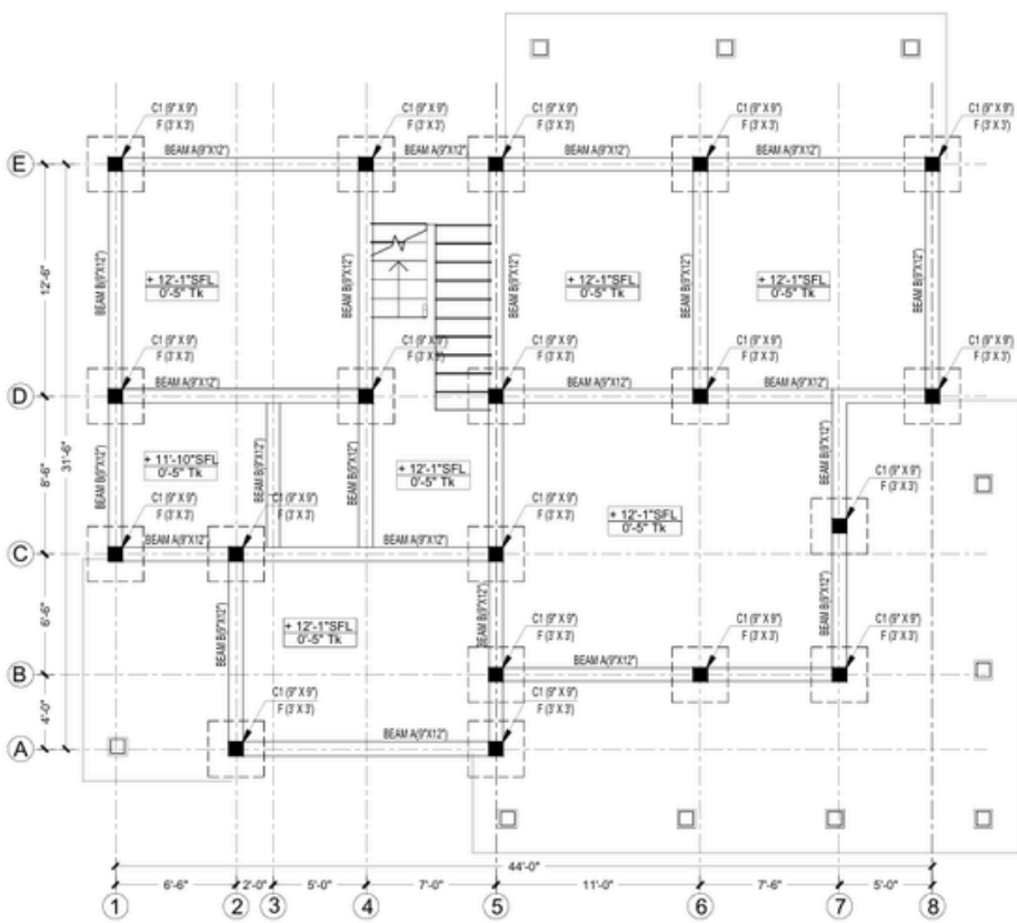
BEAM & COLUMN LAYOUT GROUND FLOOR scale 1/4"=1'0"
